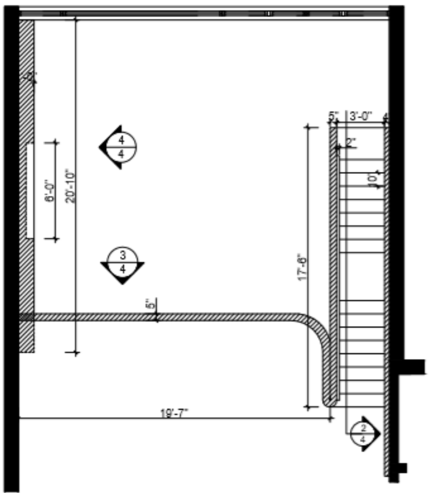
1 4 STAIR & RAILING PLAN SCALE: 1/4" = 1'-0"
